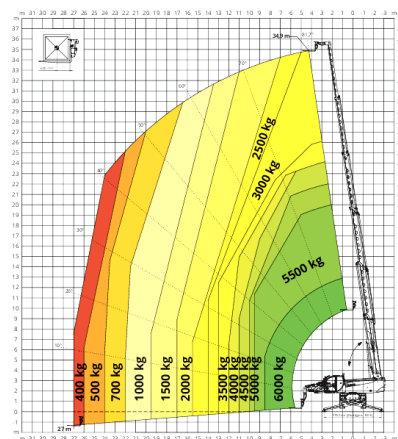
360° LOAD CHART ON FULLY EXTENDED STABILIZERS
