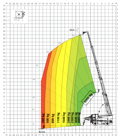
FRONTAL LOAD CHART ON TYRES
