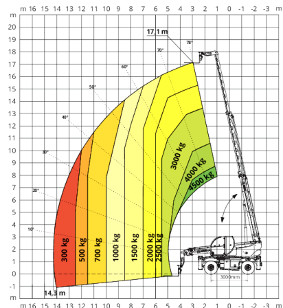
WINCH 5,000 kg
